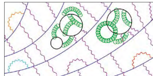
Freewheelin’ Artistic sketch of muons (blue) interacting with a magnetic field (purple), including “ g-2 ” contributions, which are the subject of intense theoretical efforts (p25).
