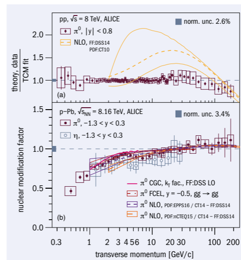
Fig. 1. (a) Neutral pion cross section compared to NLO pQCD calculations in pp collisions at 8 TeV, normalised to a phenomenological two-component model (TCM) fit of the data. (b) Nuclear modification factor of \pi^0 and \eta mesons in p–Pb collisions at 8.16 TeV compared to calculations based on NLO pQCD with nuclear PDFs, the Color Glass Condensate (CGC) framework, and pQCD with final-state energy loss (FCEL).
