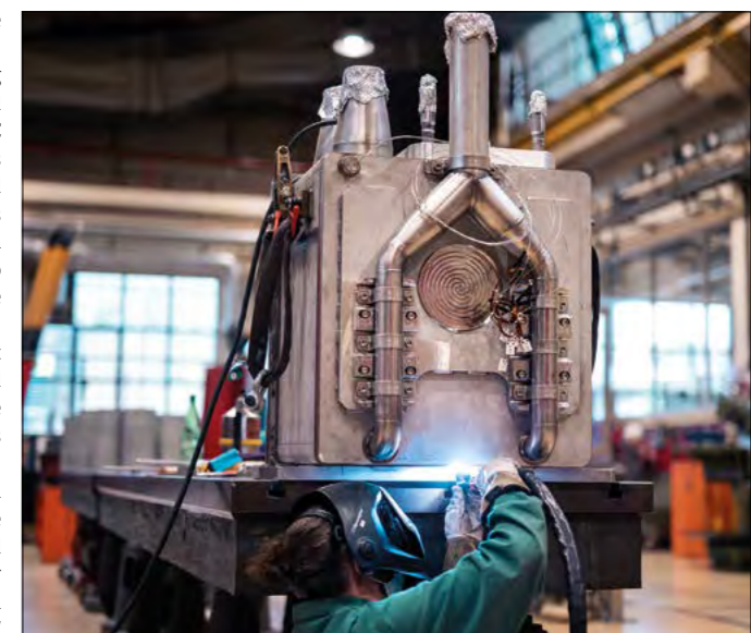
Neutron production target Welding of the upstream cover and proton window on n_TOF’s third generation lead-based neutron spallation target.
