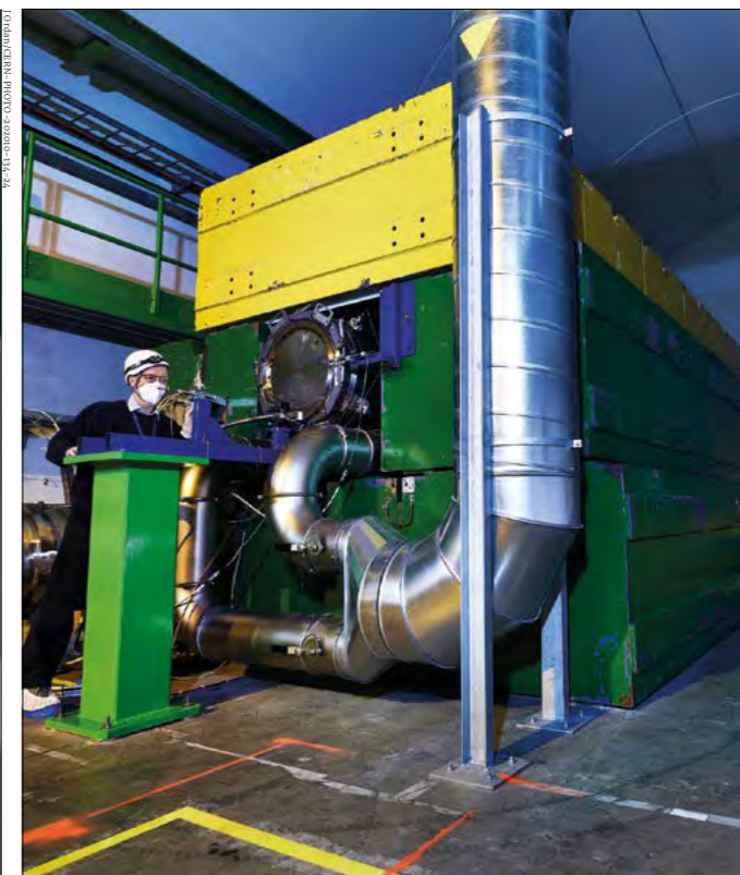
End of the line The upgraded LHC beam dump, capable of absorbing 560 MJ of kinetic energy in a period of 86 \mu s, installed in its shielding in March 2021.
