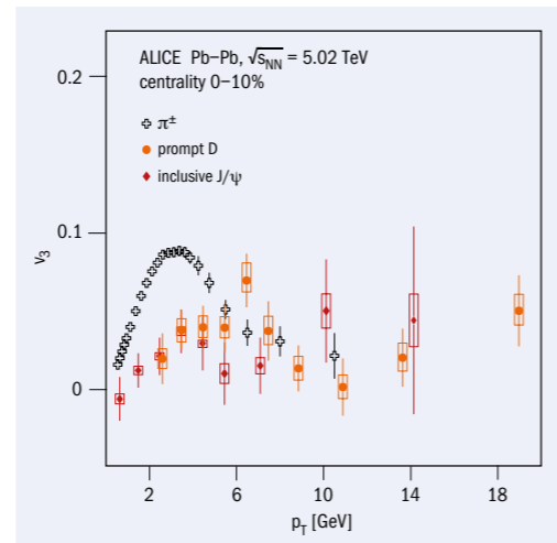
Triangular flow ALICE measurements of differential triangular-flow coefficients for charged pions, D mesons and J/ψ mesons in central (0–10% centrality) lead-lead collisions at 5.02 TeV.
